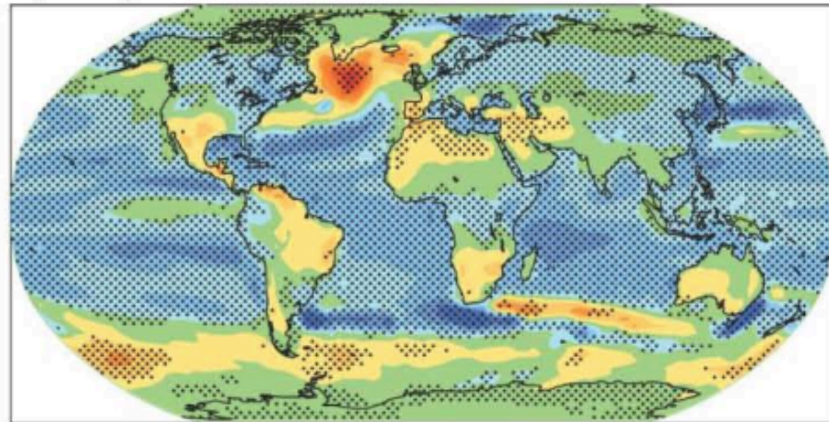
d) Evaporation
