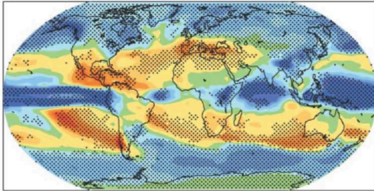
a) Precipitation
