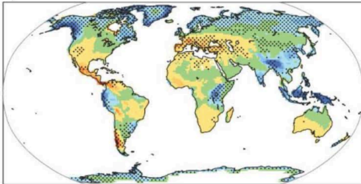
c) Runoff
